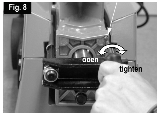
Bleed screw
